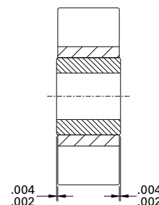
FIGURE K – IDLER BUSHING PROTRUSION
